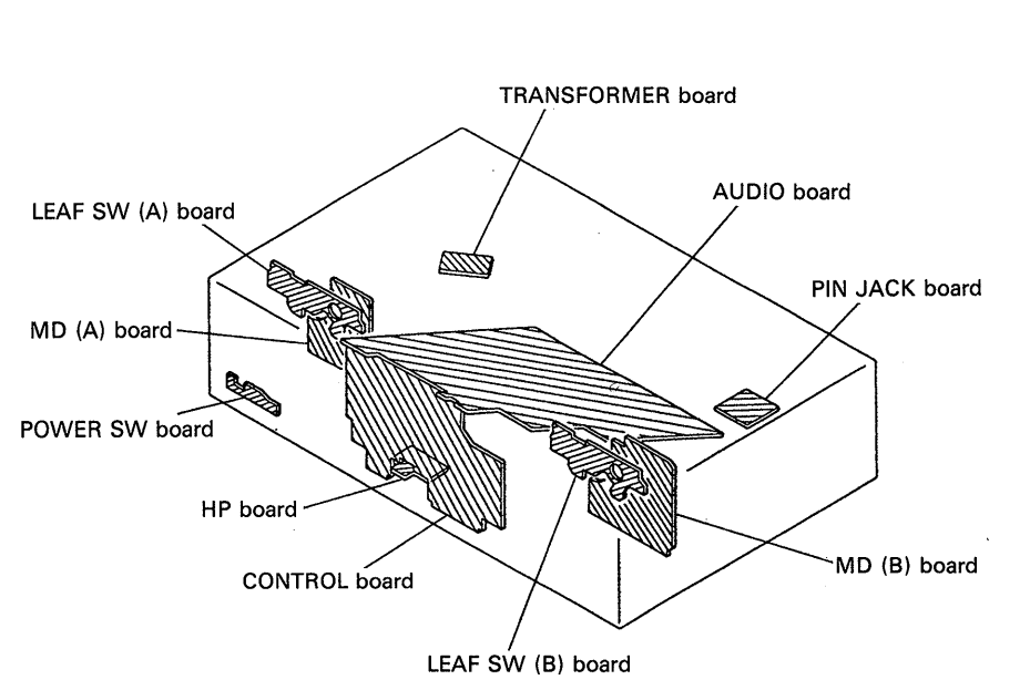
4-4. CIRCUIT BOARDS LOCATION
