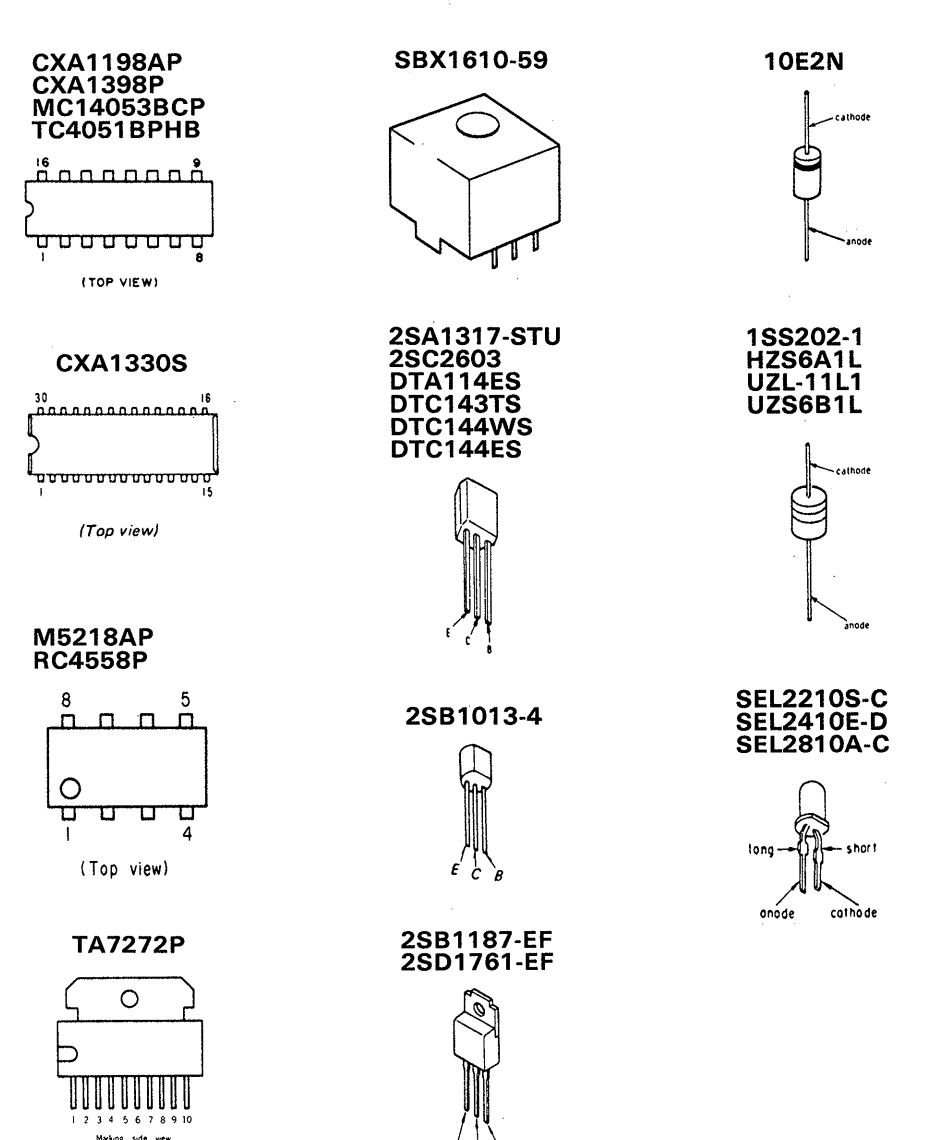
4-5. SEMICONDUCTOR LEAD LAYOUTS
